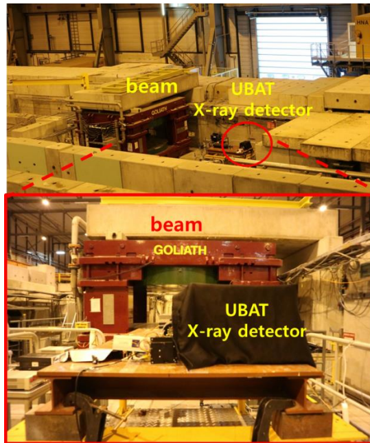
Figure 5: Test set up at H4 beam line of CERN. The dark box which includes X-ray detector is placed in front of beam line.
