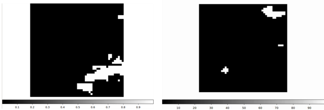
Figure 7. 48×48 channels X-ray hitmap in space. A white color is X-ray hitting channel and black is no X-ray channel. Left: One of 700 frames data on Sep.29,2016. Exposure time is 1msec. Right: One of 700 frames data Nov.24, 2016. Exposure time is 1msec.
