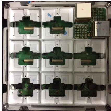
Figure 4: The mini X-ray detector of UBAT for ground test. There is an analog electronics, 2 YSO scintillation crystals and MAPMTs set on right-upper side of the UBAT detector structure.
