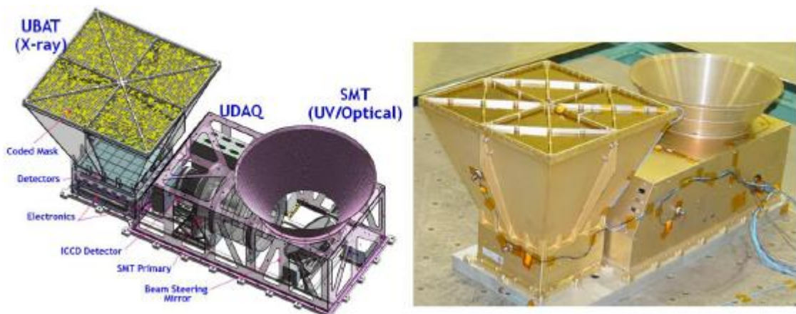
Figure 1: A composition of UFFO-pathfinder (left) and assembled flight model (right)[1]
