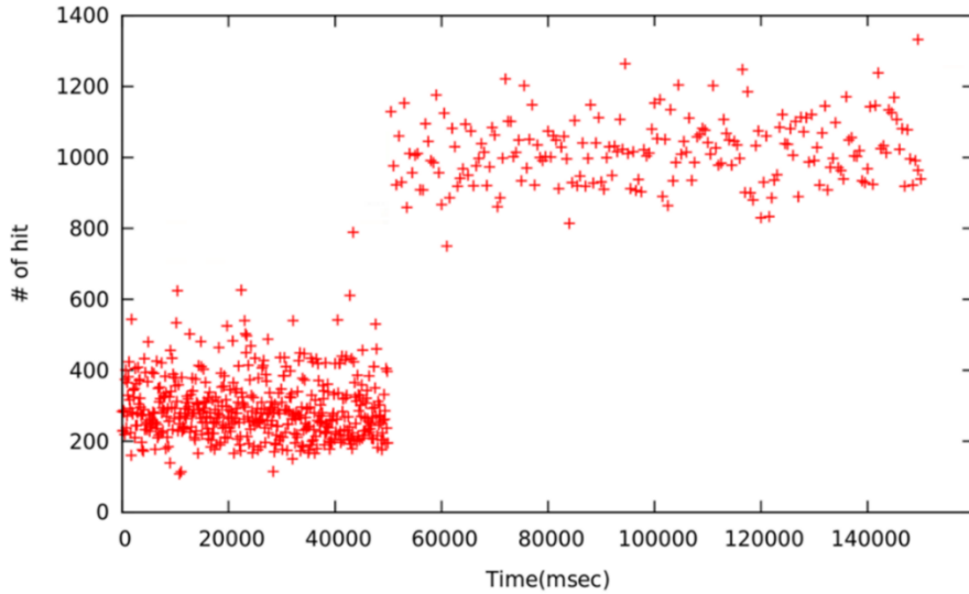
Figure 3: Number of hit of each frame on July 5,2016 data
