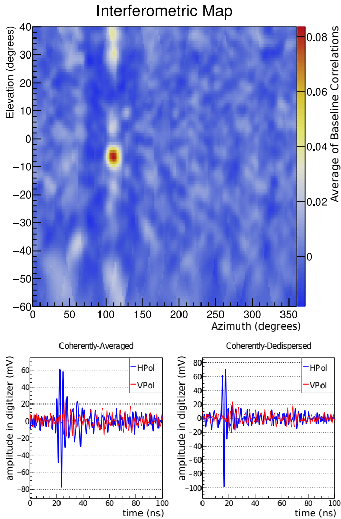
FIG. 4. An example of an interferometric map (top), a coherently-averaged waveform (bottom left), and a de-dispersed coherently-averaged waveform (bottom right) for a calibration pulser event. The color scale in the top panel corresponds to the normalized cross-correlation value. Although we expect Askaryan neutrino signals to be mostly vertically polarized, the calibration pulser is horizontally polarized.
